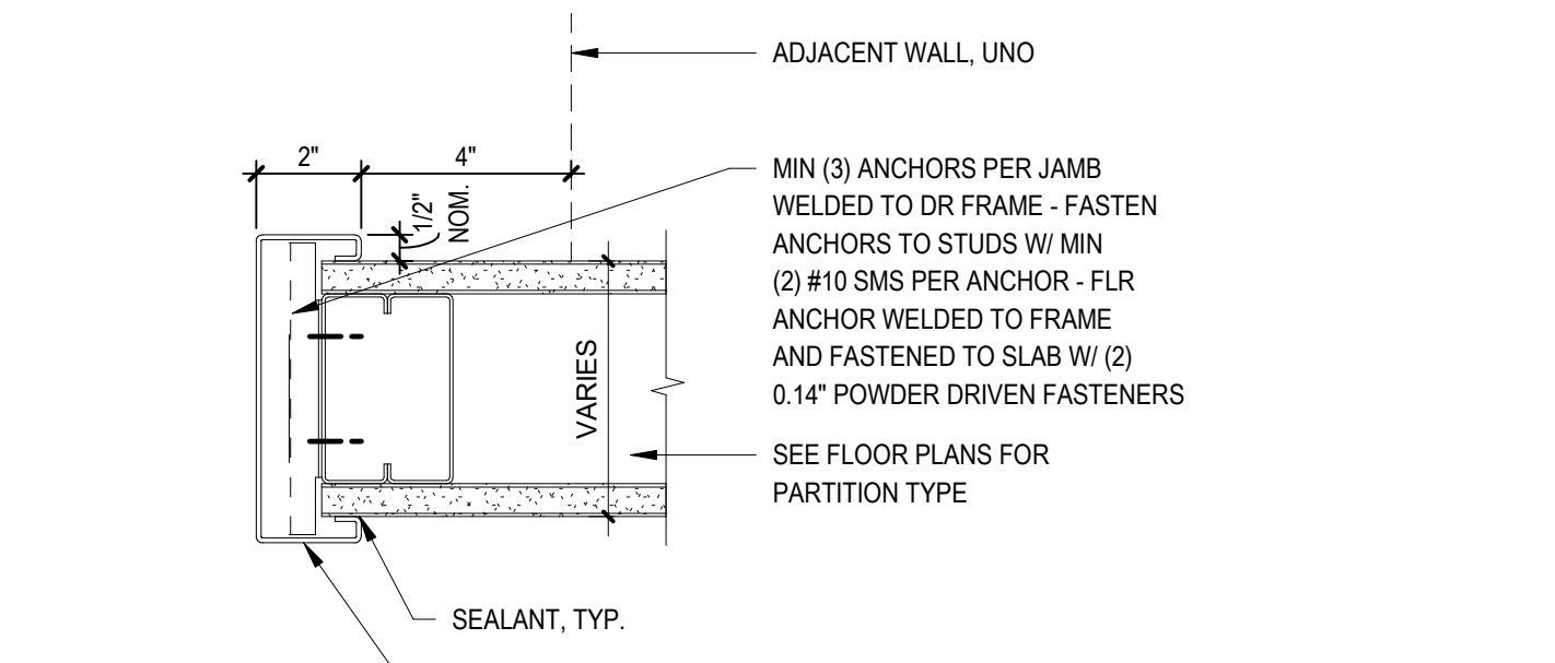
D2 FRAME TYPE: S - HM CASED OPEN JAMB 3" = 1'-0"
