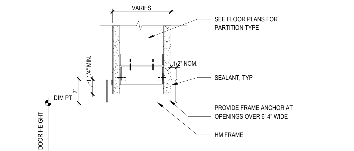
C1 FRAME TYPE: S - HM DOOR HEAD 3" = 1'-0"
