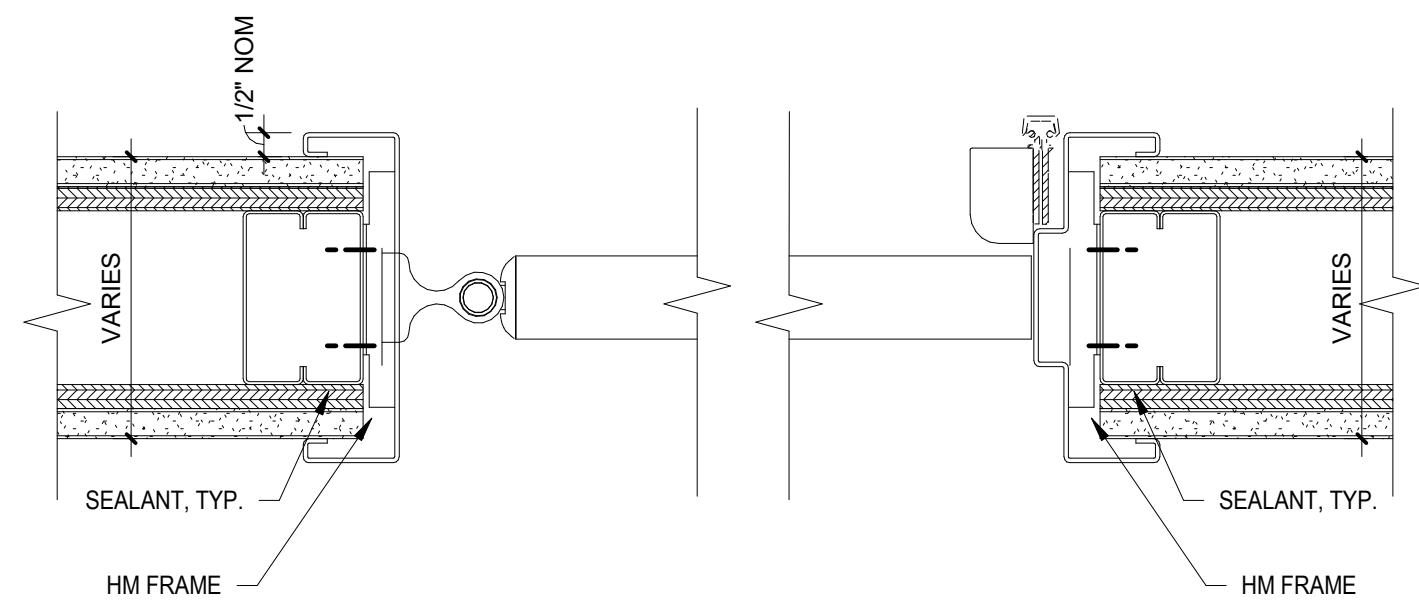
D1 FRAME TYPE: ANT-BARRICADE - HM DOOR JAMB 3" = 1'-0"
